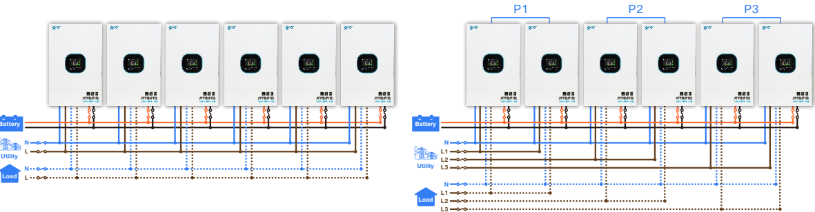
Parallel Operation in Single phase
